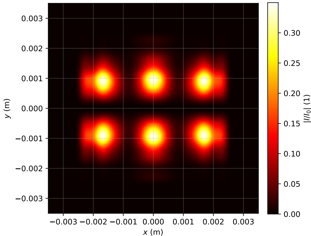
Intensity profile I(x, y, z = 3.901)/I_0 , P_{in}=3.0P_{cr} , artificial time
